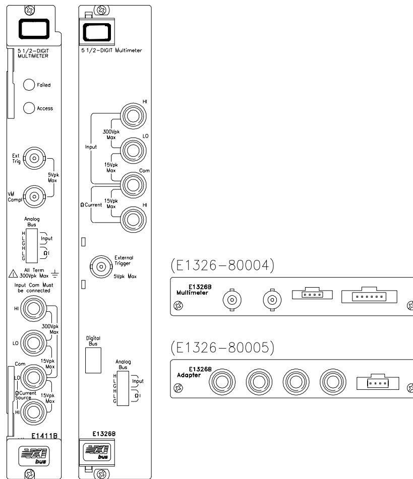
Figure 2-7. Agilent E1326B/E1411B Input Terminals
